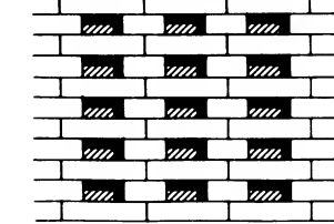
27 As 25 (holes 1/4 x 1/2 brick)
